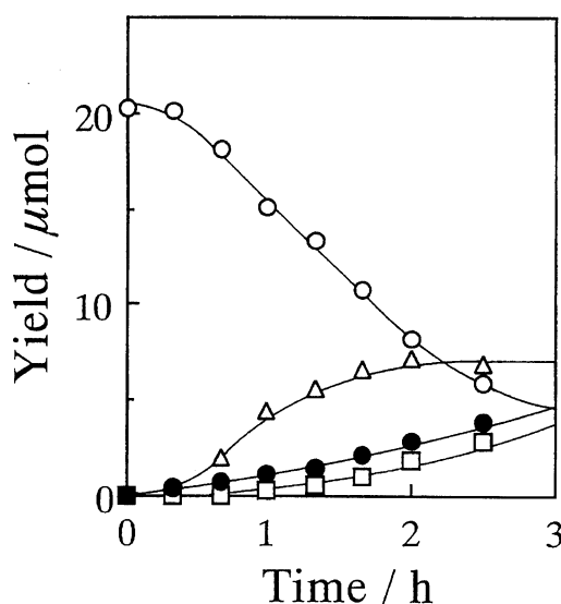
Fig. 1. Time-conversion plots for CdS-photocatalyzed isomerization and reduction of dimethyl maleate by TEA in methanol: (○) dimethyl maleate, (△) dimethyl fumarate, (□) dimethyl succinate, and (●) DEA.
